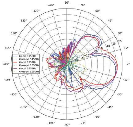
Elevation, Vertical
